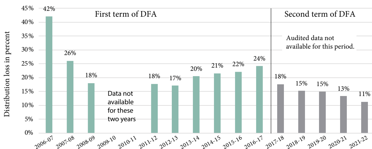
Figure 1: Distribution Loss Reduction Trajectory for Bhiwandi
